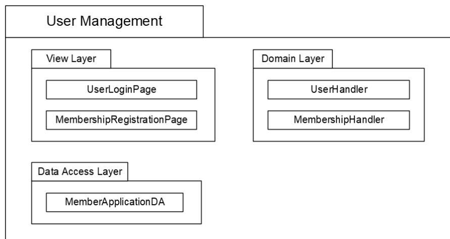
Figure 4.5 Package Diagram 1 for User Management Subsystem
