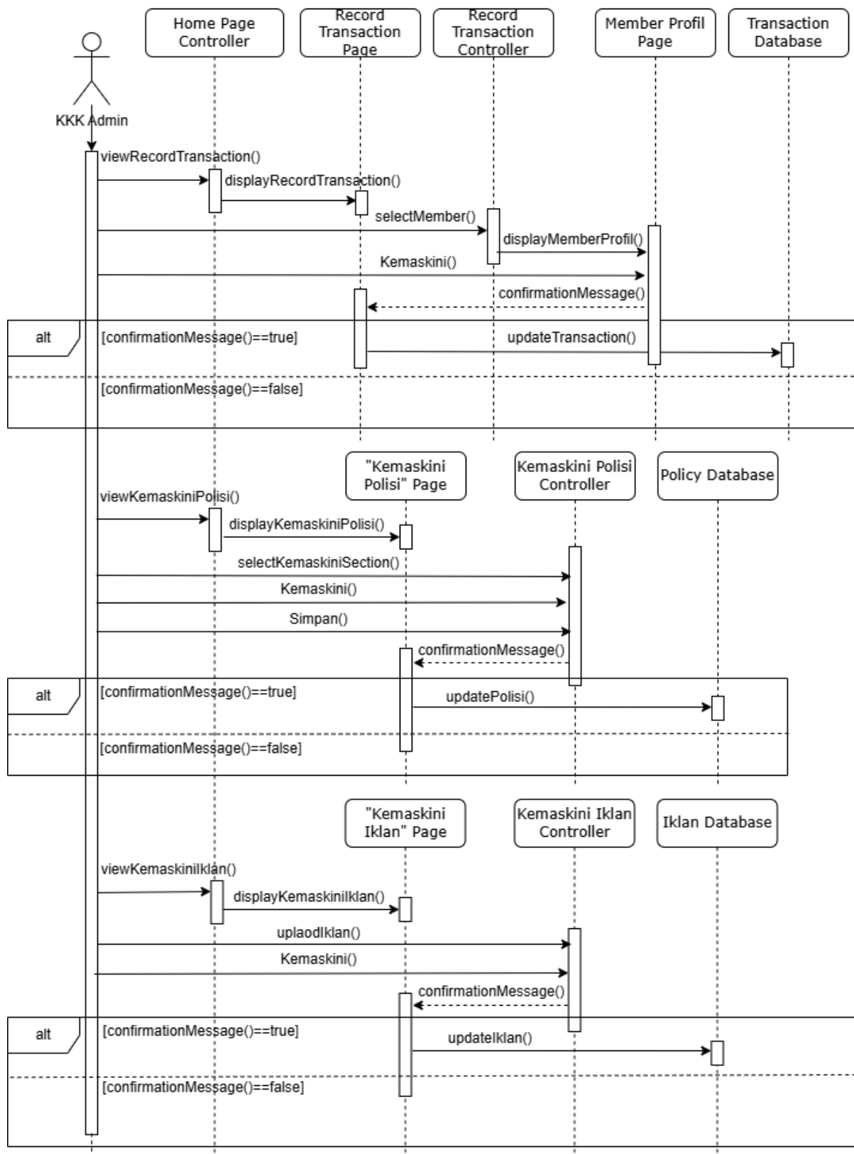
Figure 4.28: SD011 Sequence Diagram for Manage System
