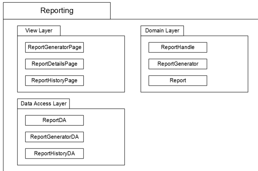
Figure 4.10 Package Diagram 6 for Reporting Subsystem
