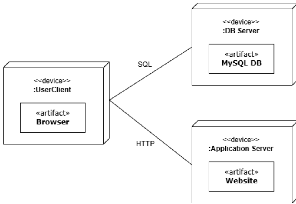
Figure 4.30: Deployment diagram for KKK Online System
