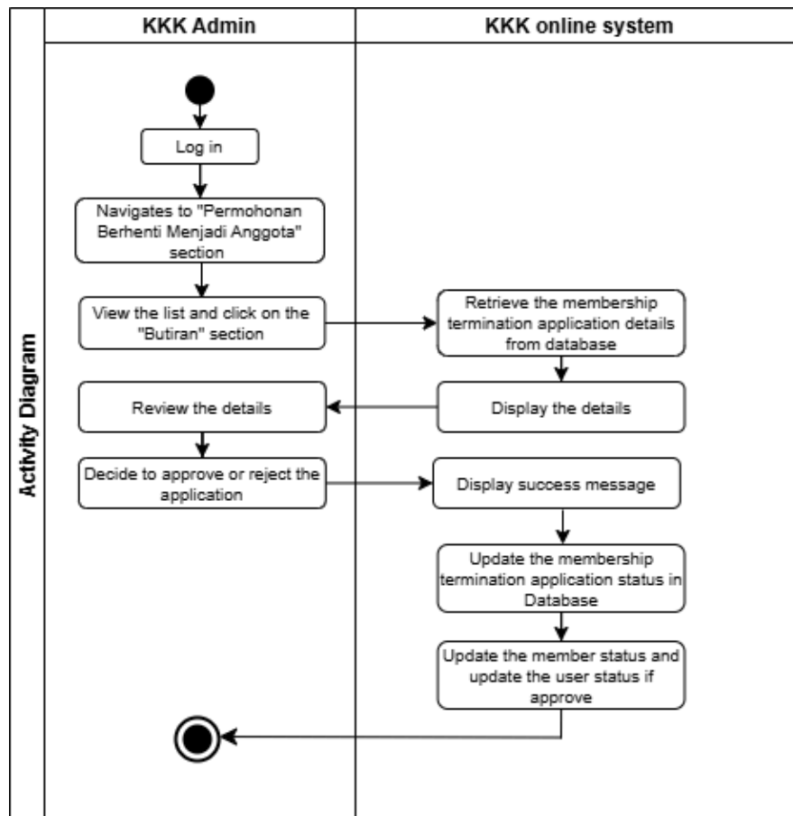
Figure 2.28 Activity Diagram for Approve Membership Termination
