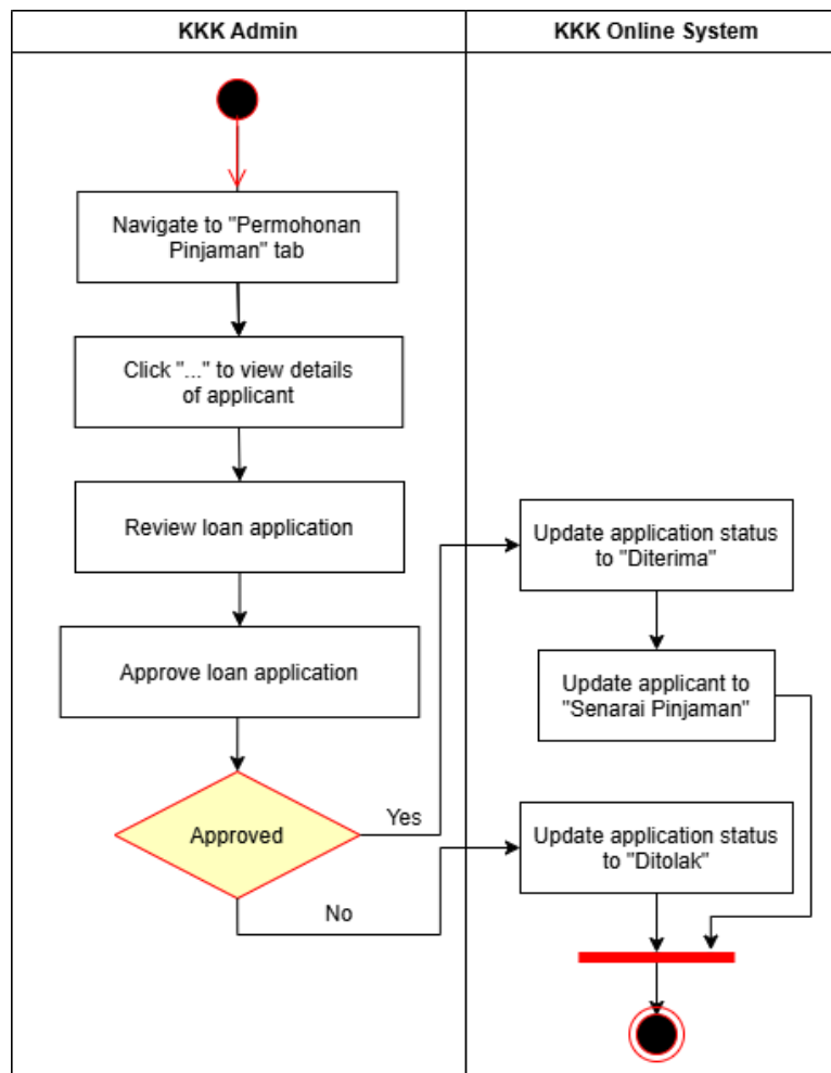
Figure 2.22: Activity Diagram for KKK Admin Approve Loan Application
