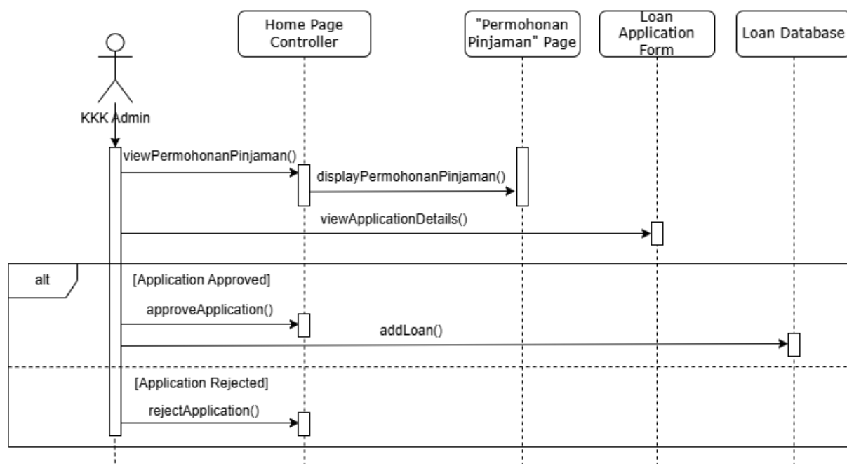
Figure 2.21: Sequence Diagram for KKK Admin Approve Loan Application
