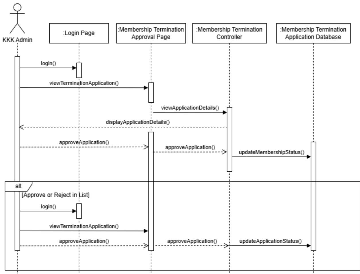
Figure 2.27: Sequence Diagram for Approve Member Termination
