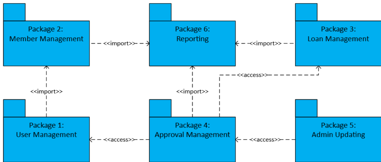
Figure 4.4 Package Diagram for KKK Online System
