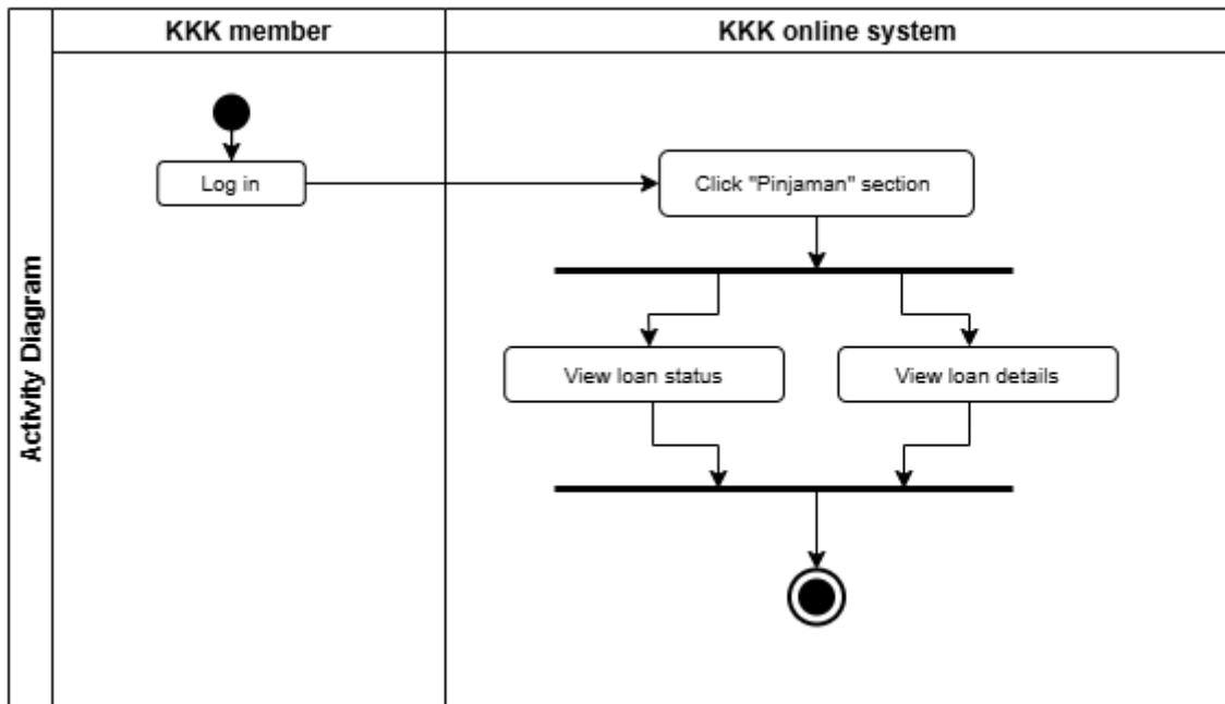
Figure 2.10: Activity Diagram for Member View Loan Application Status
