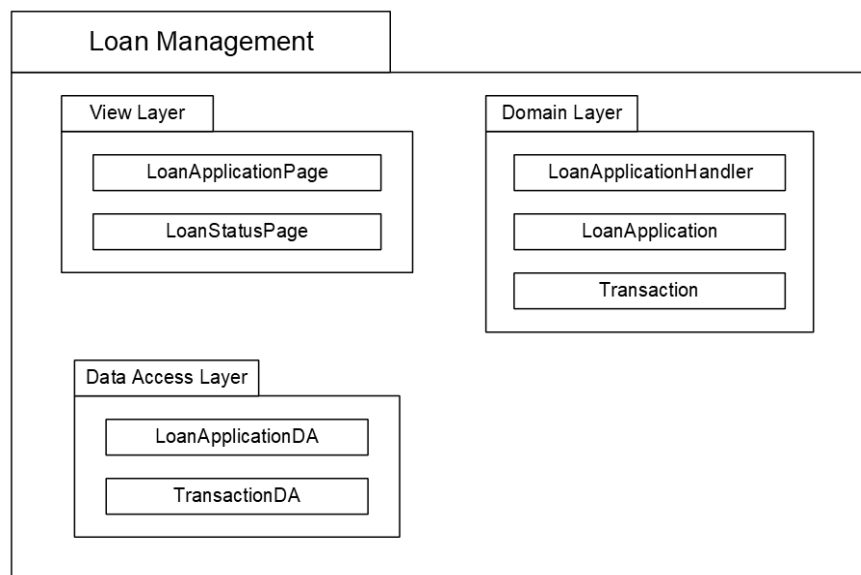
Figure 4.7 Package Diagram 3 for Loan Management Subsystem
