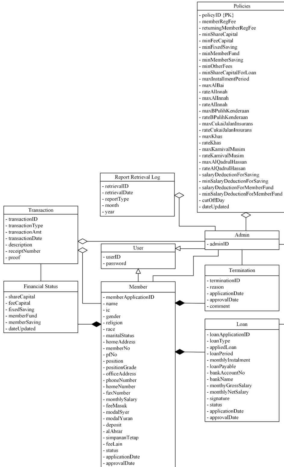
Figure 4.17 Class Diagram for Admin Reporting Module
