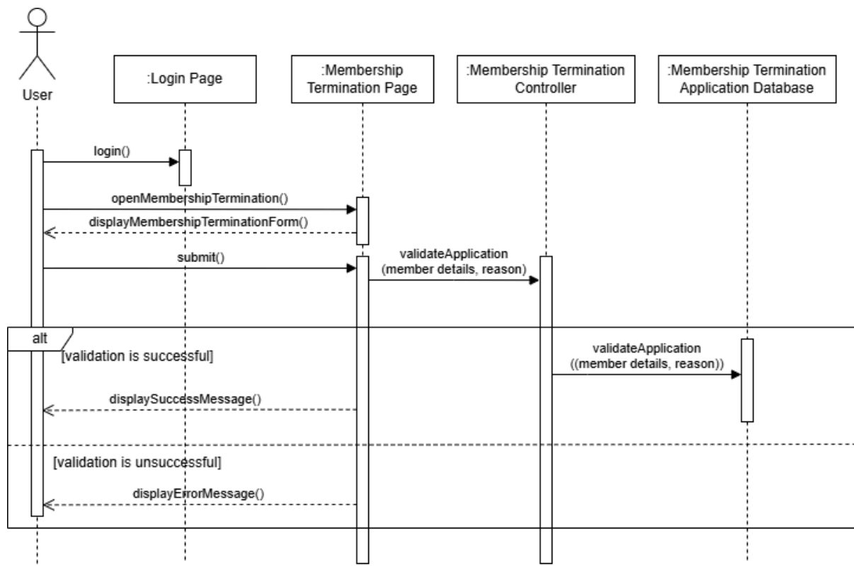
Figure 4.24: SD007 Sequence Diagram for Apply Membership Termination
