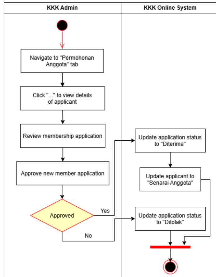
Figure 2.20: Activity Diagram for KKK Admin Approve New Member Application
