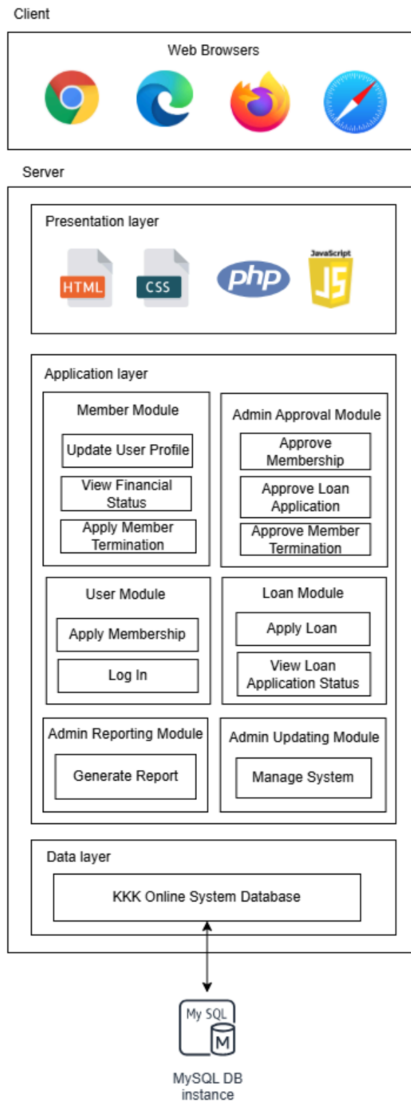
Figure 4.3 Architecture Diagram for KKK Online System
