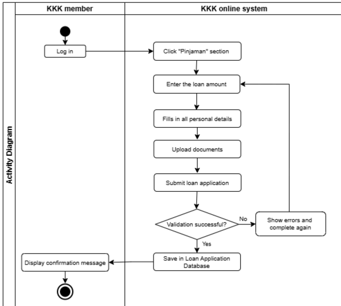
Figure 2.8: Activity Diagram for Member Apply for a loan
