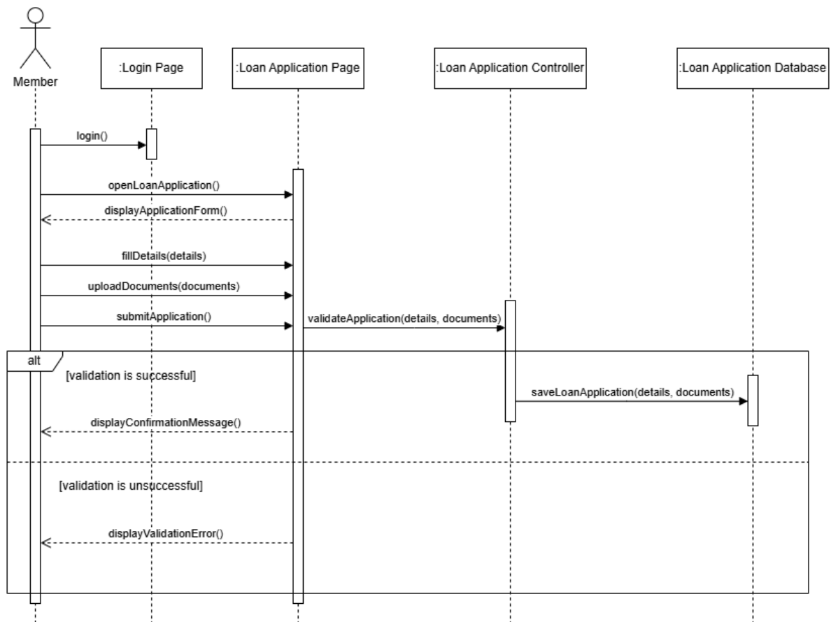
Figure 2.7: Sequence Diagram for Member Apply for a Loan
