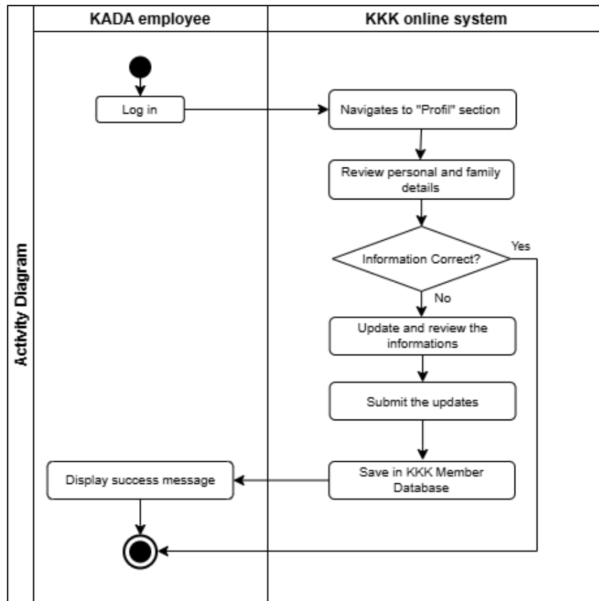
Figure 2.4: Activity Diagram for Member Update User Profile
