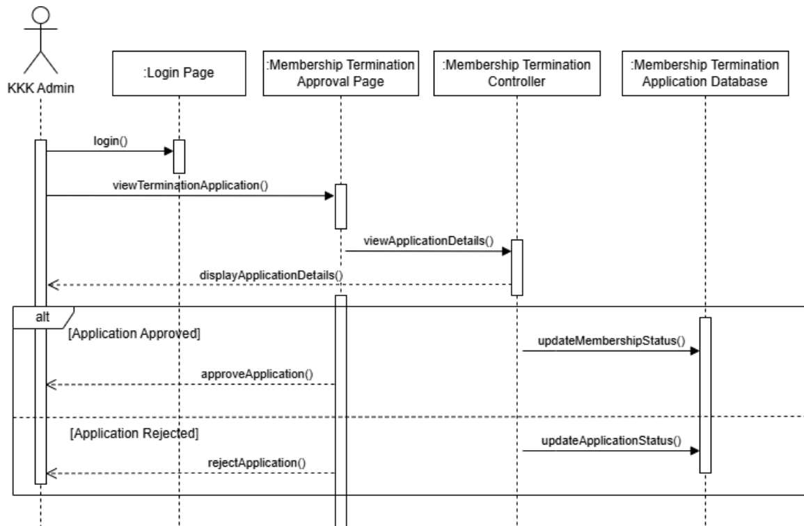
Figure 4.29: SD012 Sequence Diagram for Approve Membership Termination
