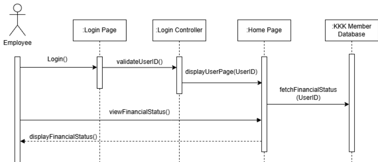
Figure 2.5: Sequence Diagram for Member View Financial Status
