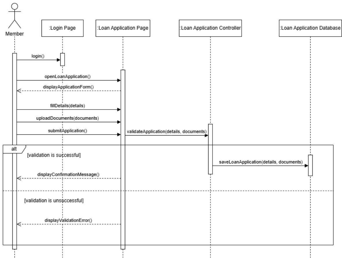
Figure 4.22: SD005 Sequence Diagram for Apply Loan
