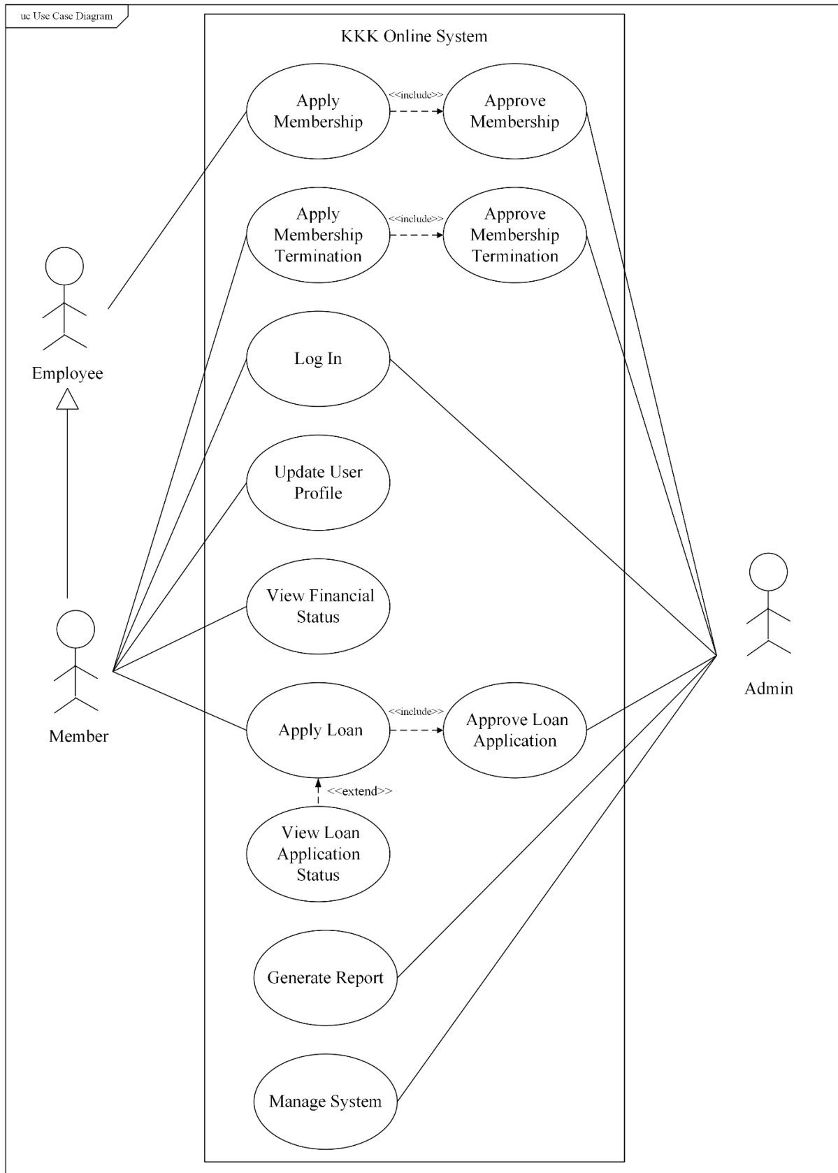
Figure 4.2 Use Case Diagram for KKK Online System
