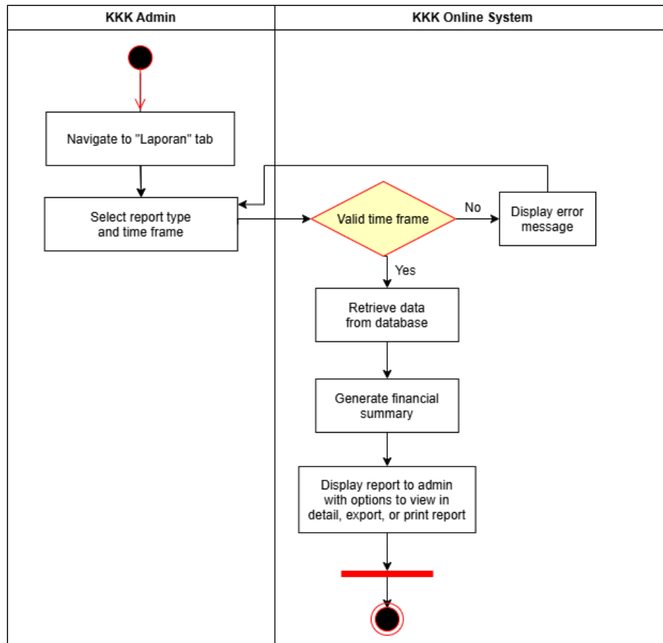
Figure 2.24: Activity Diagram for KKK Admin Generate Reports
