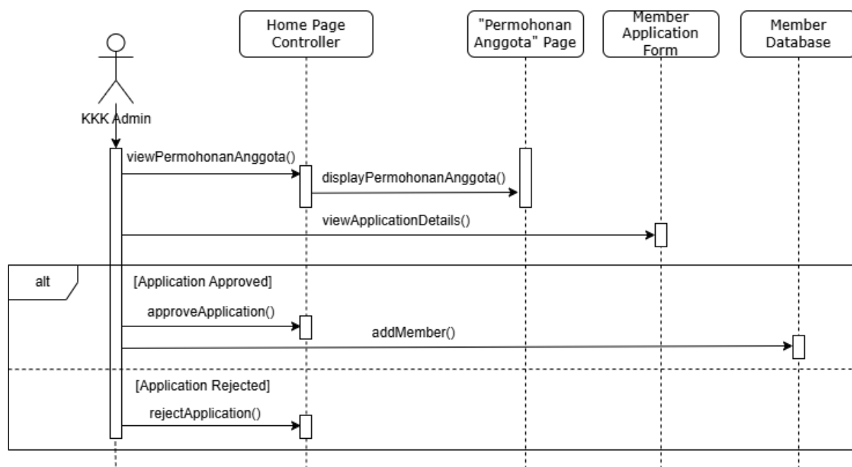
Figure 2.19: Sequence Diagram for KKK Admin Approve New Member Application
