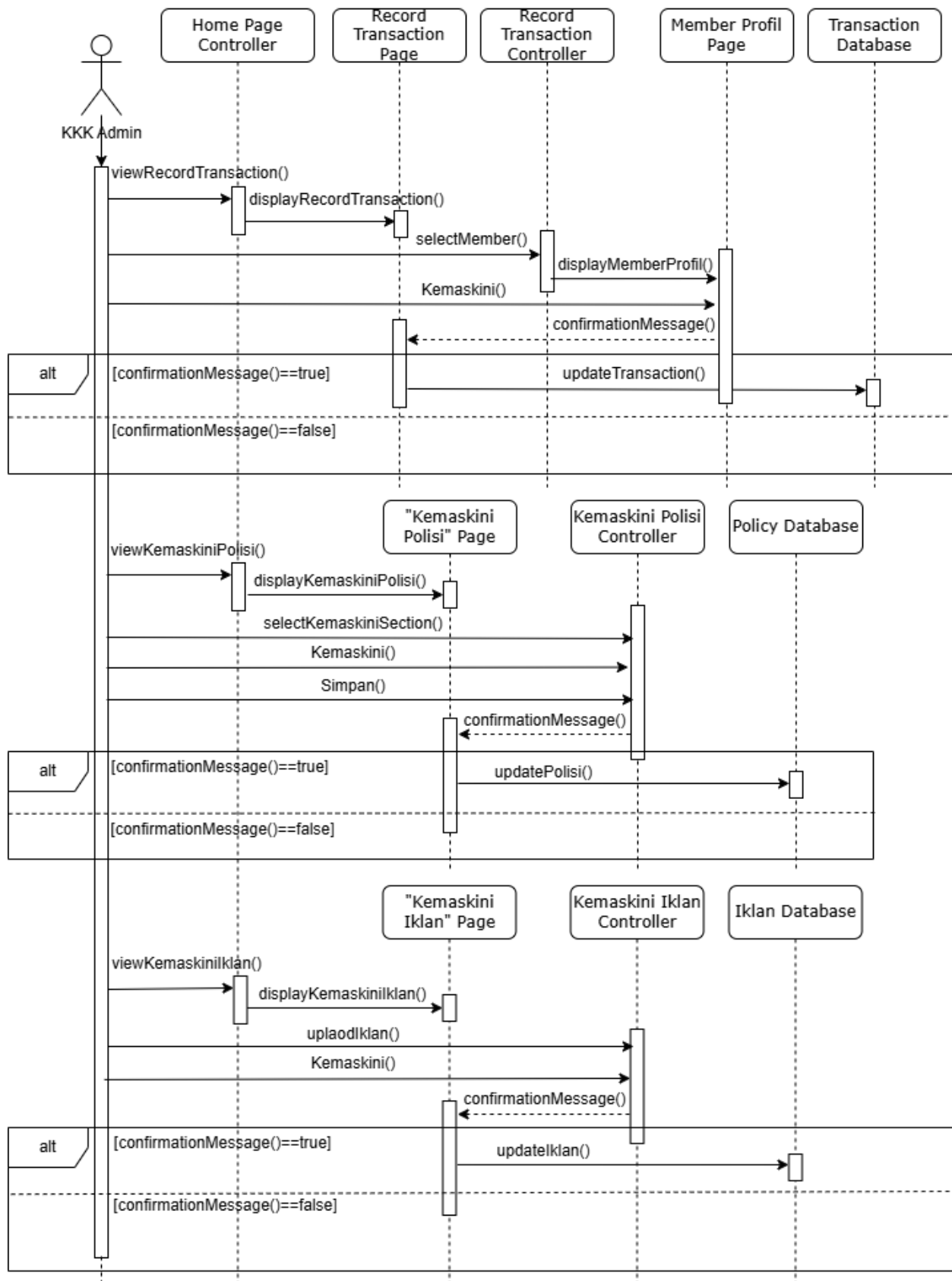
Figure 2.25: Sequence Diagram for KKK Admin Manage System
