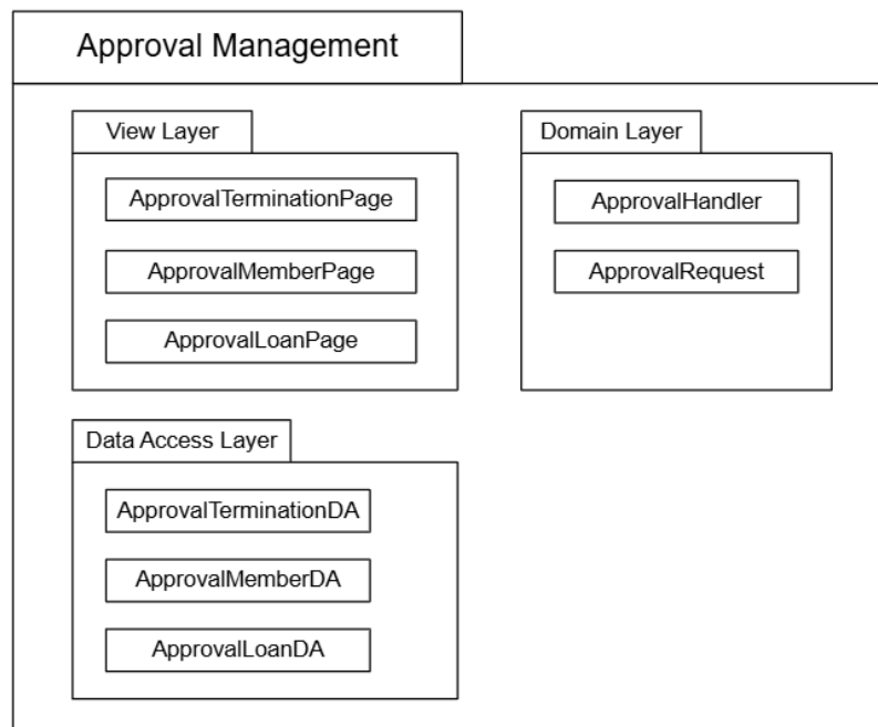
Figure 4.8 Package Diagram 4 for Approval Management Subsystem
