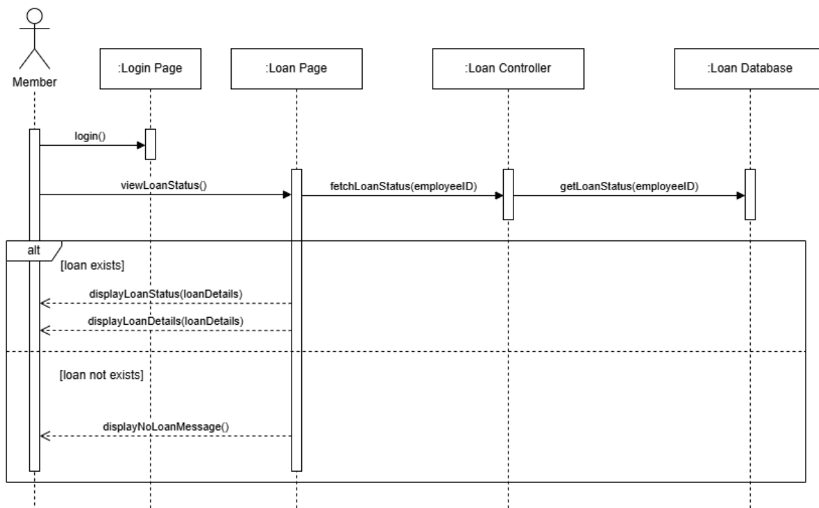
Figure 2.9: Sequence Diagram for Member View Loan Application Status
