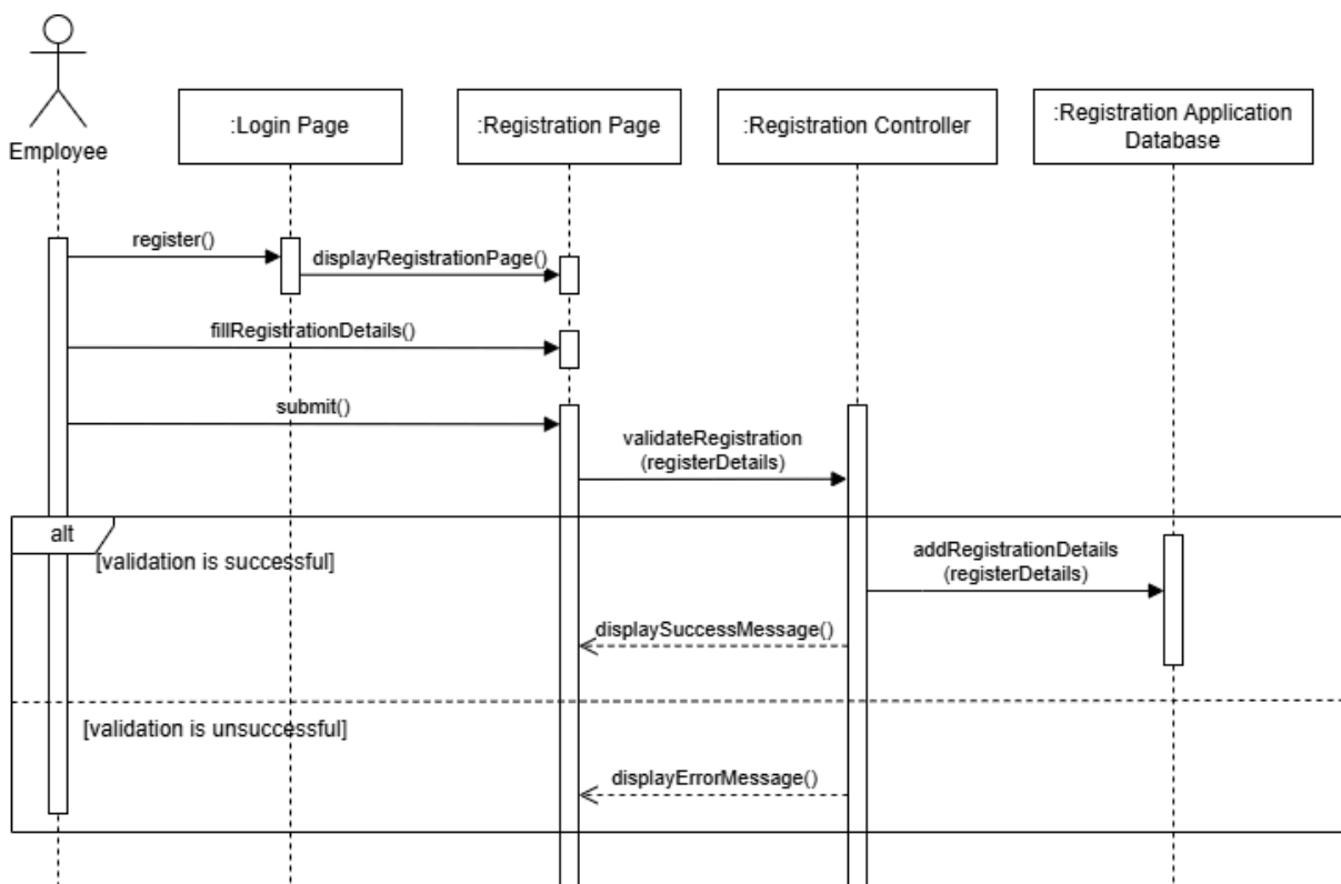
Figure 2.1: Sequence Diagram for KADA Employee Apply Membership
