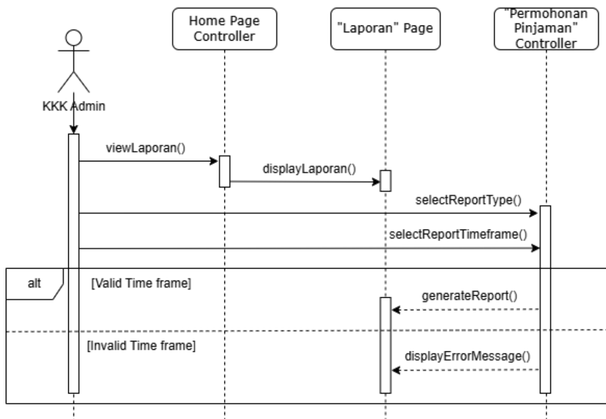
Figure 2.23: Sequence Diagram for KKK Admin Generate Reports
