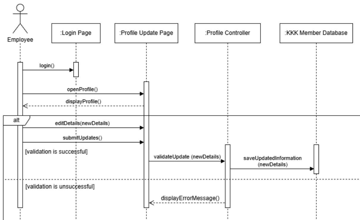
Figure 2.3: Sequence Diagram for Member Update User Profile
