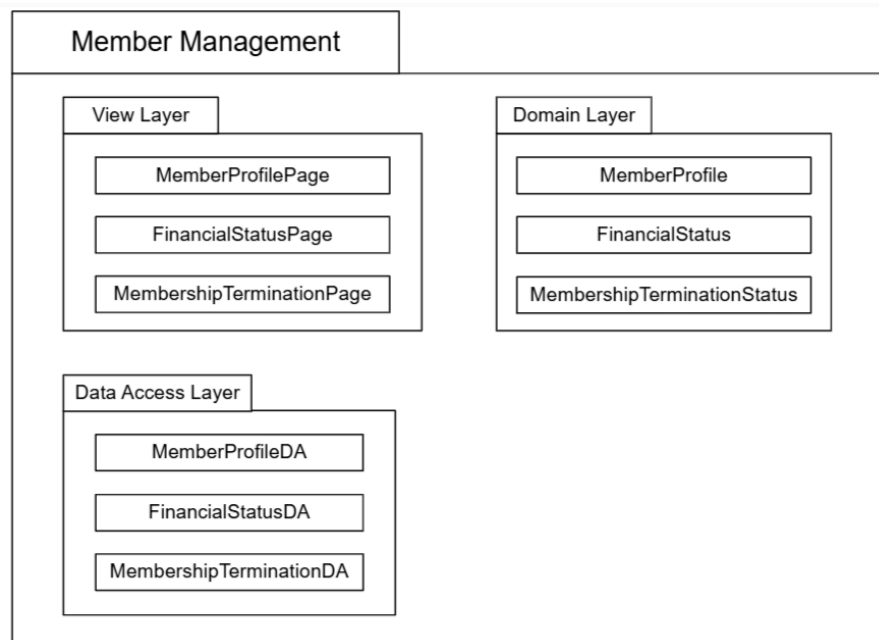
Figure 4.6 Package Diagram 2 for Member Management Subsystem
